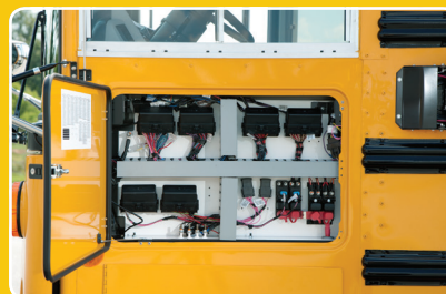
Exterior electrical access compartment for easy troubleshooting and service.
